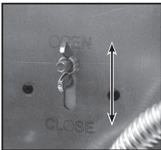
Figure 67: Venturi adjustment.
