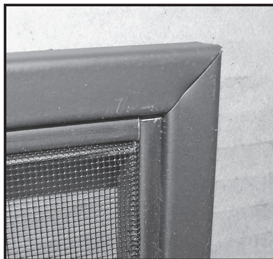
Figure 54: Front side of screen mesh.
