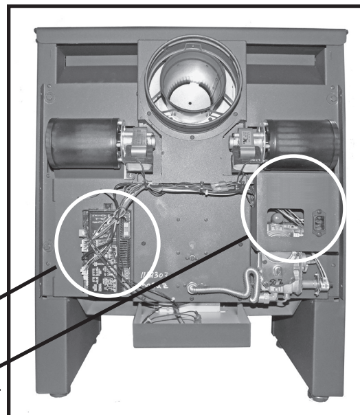
Figure 65: IFC module location.
