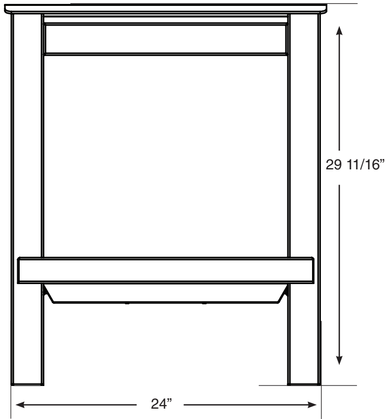
Figure 21: TN24 dimensions.
