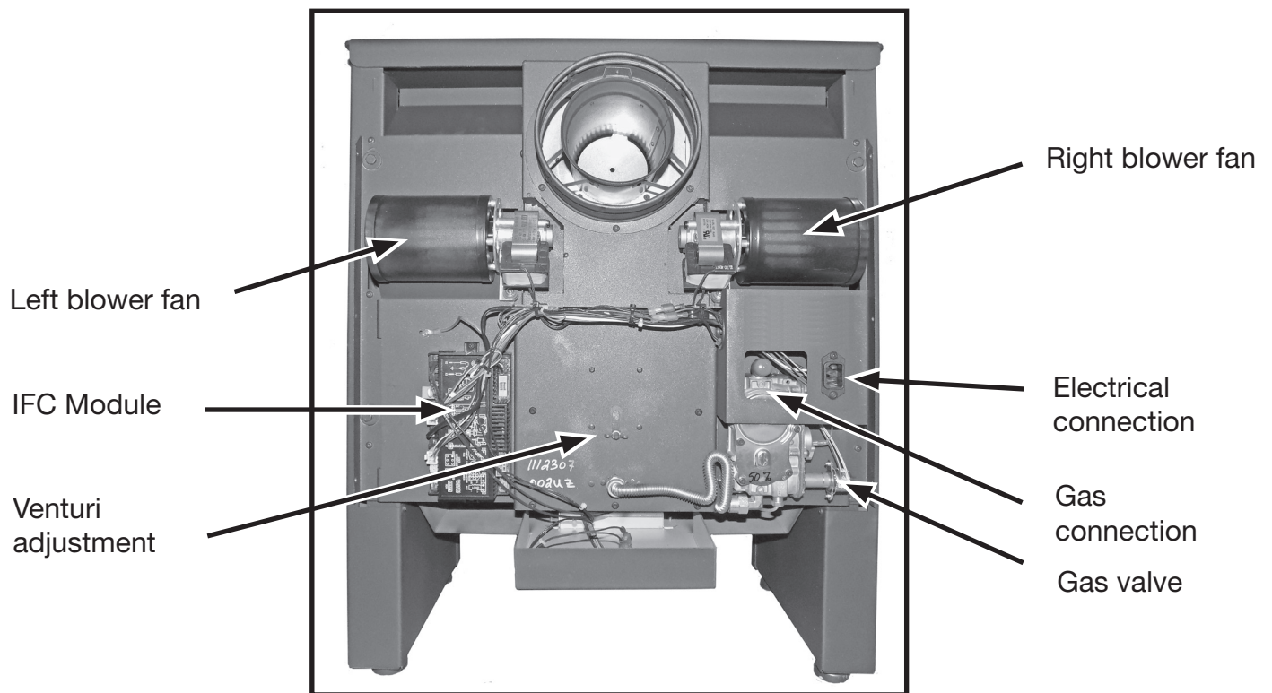
Figure 31: TN24 rear side components.
