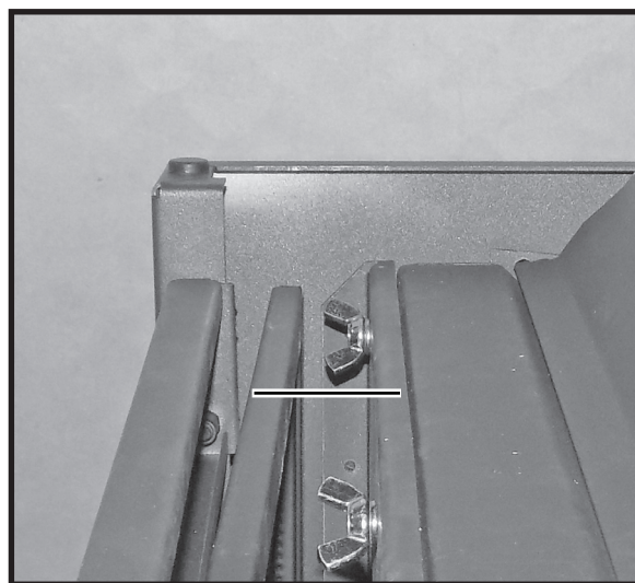
Figure 56: proper orientation of screen mesh.
