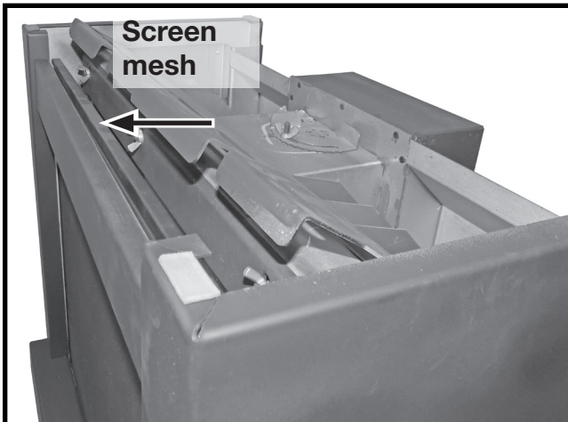
Figure 58: Screen mesh holder.
