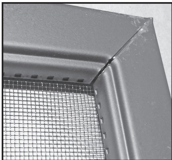
Figure 53: Rear side of screen mesh.
