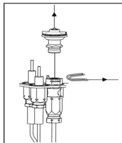
Figure 72: Pilot hood removal.
