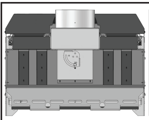
Figure 66: TN24 Damper.
