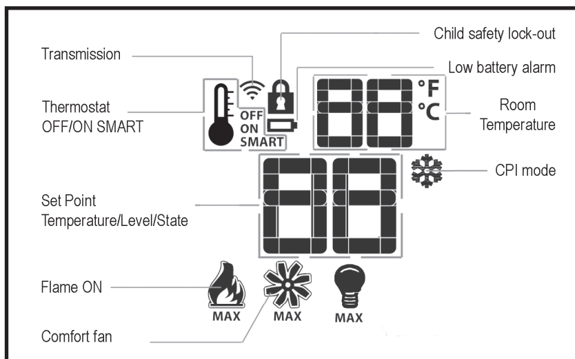
Figure 2: Proflame 2 remote transmitter screen detail.
